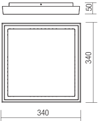
Dimension
