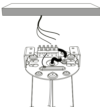
Collegamento 1-10V - 1-10V diagram
