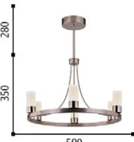
5004-46 Ø 590 ↑ 630 ↓ G9 220V 6 x 40W IP20 metal, glass
